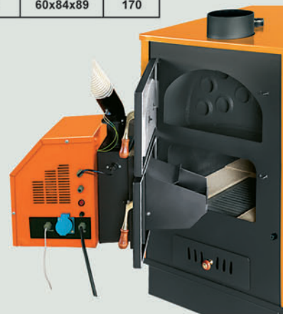
Boiler PRITY LB
