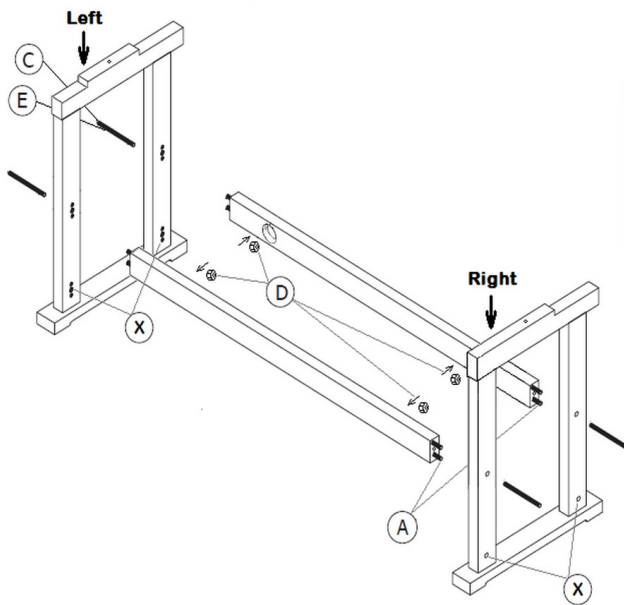
1) Base assembly
