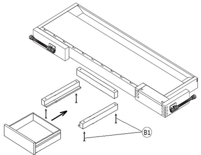
2) Drawer attaching
