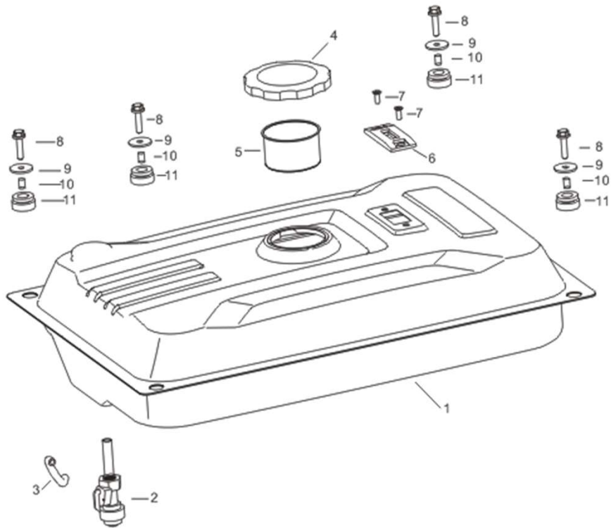
FIG.11 TANK ASSY, FUEL (F11)
